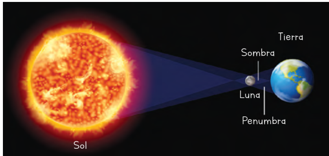
Eclipse lunar
