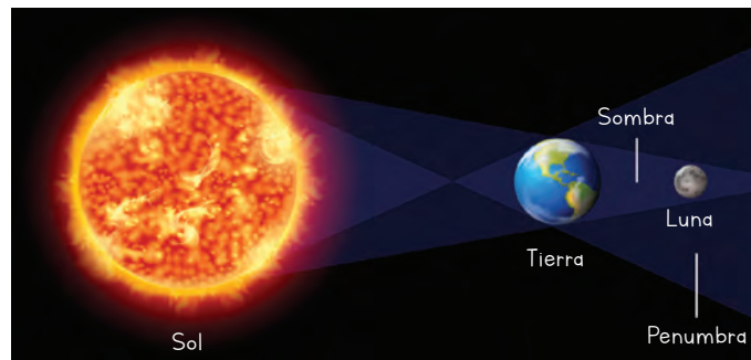
Eclipse solar
